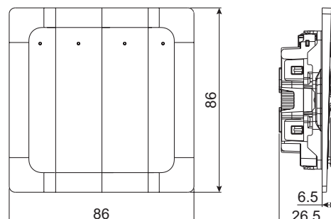
4G Switch
