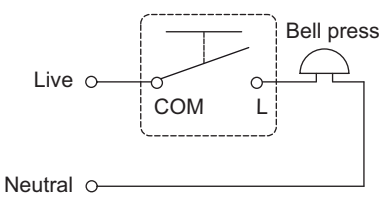
Bell Switch
