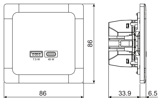
USB Chargers
