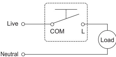
Momentary Switch
